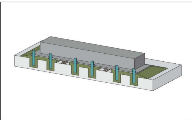
Figure 14 - Finished baseplate
