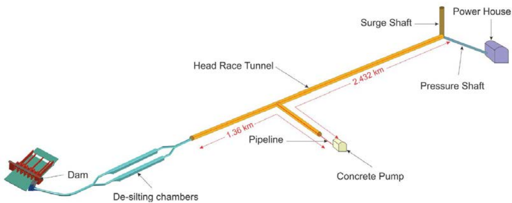
Layout of long distance concrete pumping - 1.36 km upstream and 2.432 km downstream
