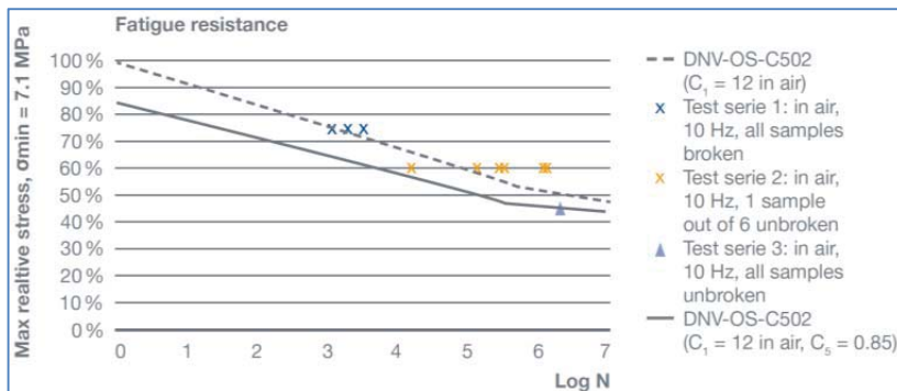
Fatigue resistance according DNV-OS-C502
