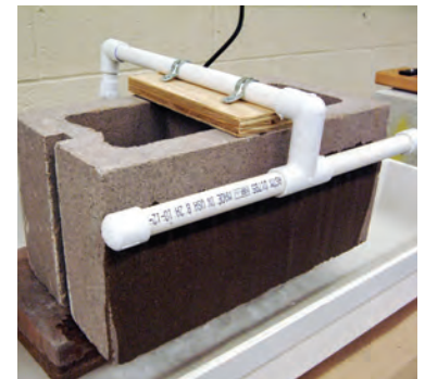
Spray-Bar Tube-test permeation of CMU
