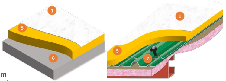
MasterSeal 550 K applied directly over Spray Polyurethane foam insulation
