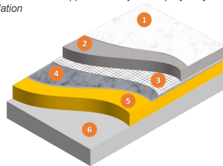
MasterSeal 550 K applied on screed for accessible roofs
